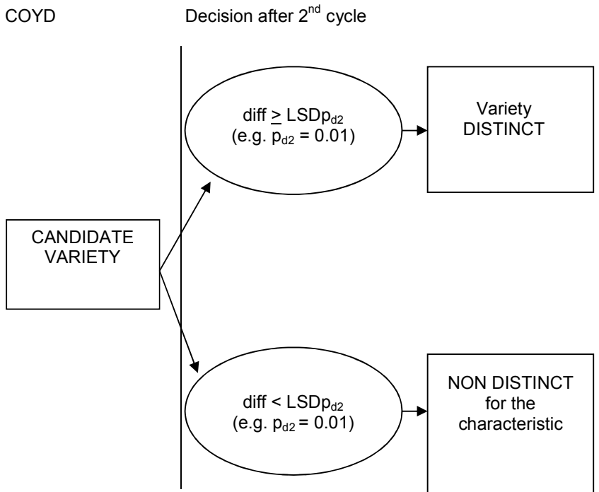
Figure 2. COYD decisions and standard probability levels ( p_i ) in Case B
